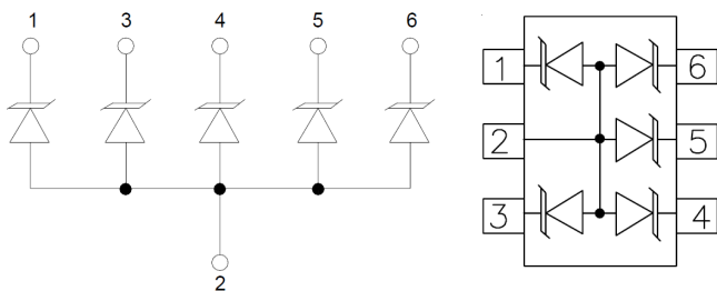
Circuit and Pin Schematic
